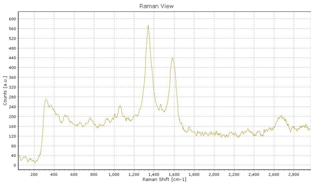
Raman Spectra
